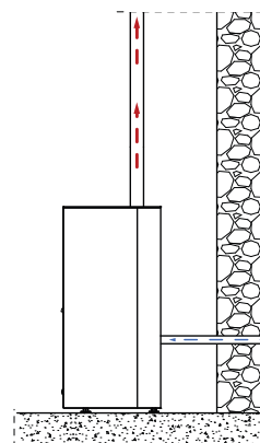
Installation Typ "b" *
